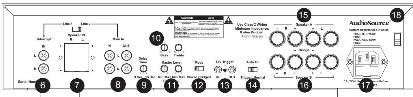
Figure 2. Rear Panel
